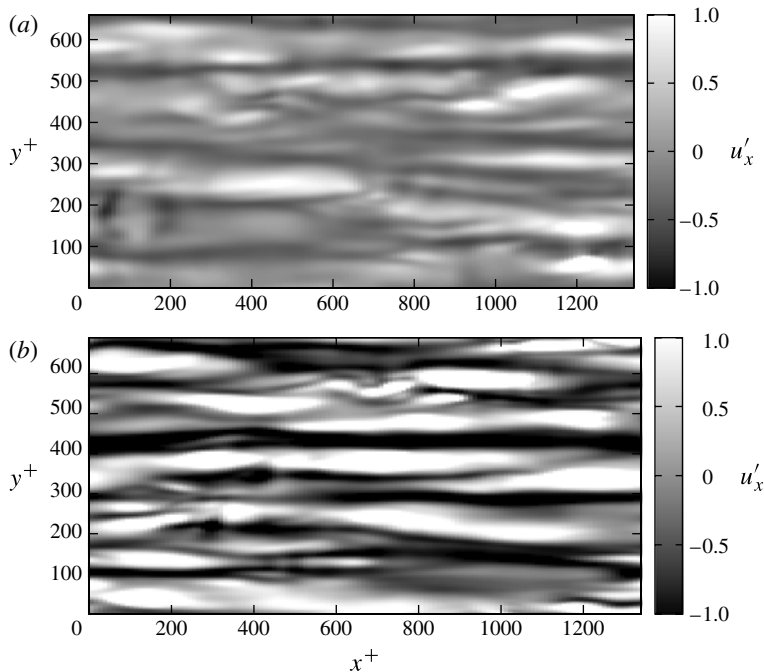
FIGURE 8. Velocity streaks in the near-wall region of the channel for flow with temperature-dependent viscosity at Re_\tau = 110 (simulation S1.3 ): (a) cold wall; (b) hot wall. Velocity contours are taken on a wall-parallel plane located at z^+ = 5 from the wall.
