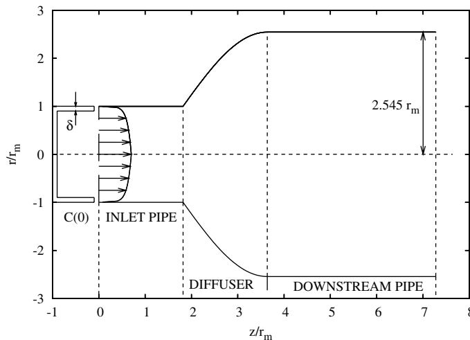
Fig. 1. Dimensions and shape of the computational domain (cross section). A turbulent, time-averaged velocity profile with shear Reynolds number of 470 is imposed at inlet. Initial particle distribution C(0) is also shown: 50% of particles used in Lagrangian tracking is initially concentrated inside the boundary-layer, in a layer \delta = 10 wall units thick. Reference frame is cylindrical, with origin on the symmetry axis ( z = 0 , r = 0 ). Third dimension is the rotation angle around the symmetry axis \theta , not shown here.
