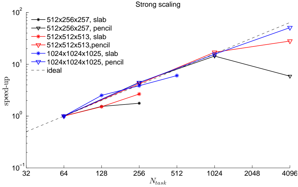
Figure 4.3: Strong scalability
